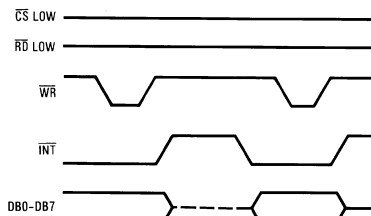
Figure 23. WR-RD Mode (Pin 7 is High) Stand-Alone Operation
